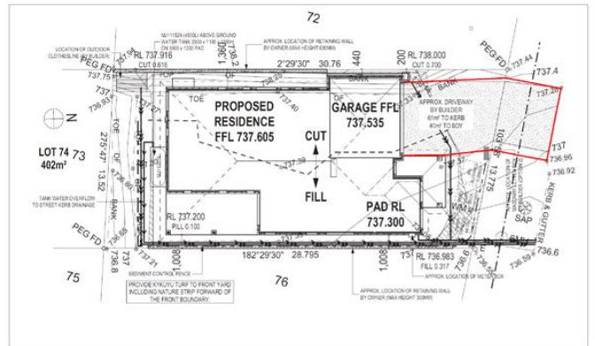
Typical Skewed Verge Crossing
