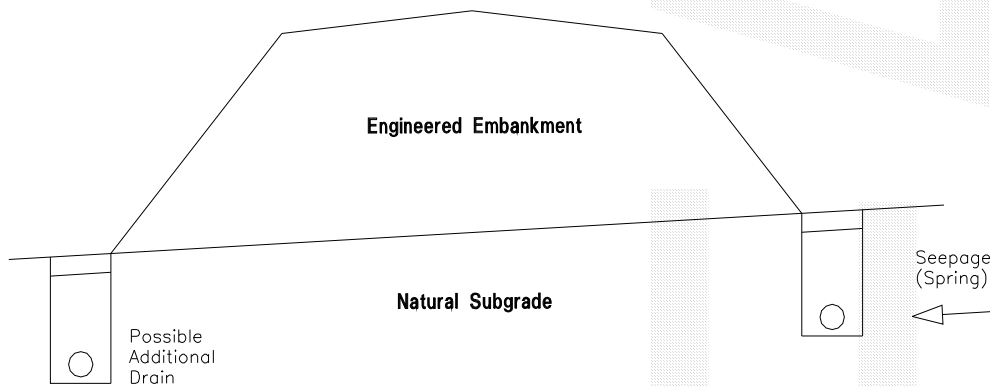
Figure D4.3 - Foundation Drains
