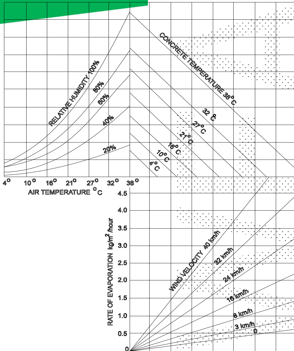
Figure C247.1 - Rate of Evaporation
