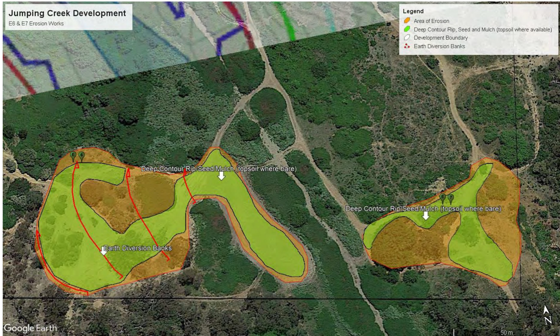
Figure 9: E6 & E7 Erosion Works
