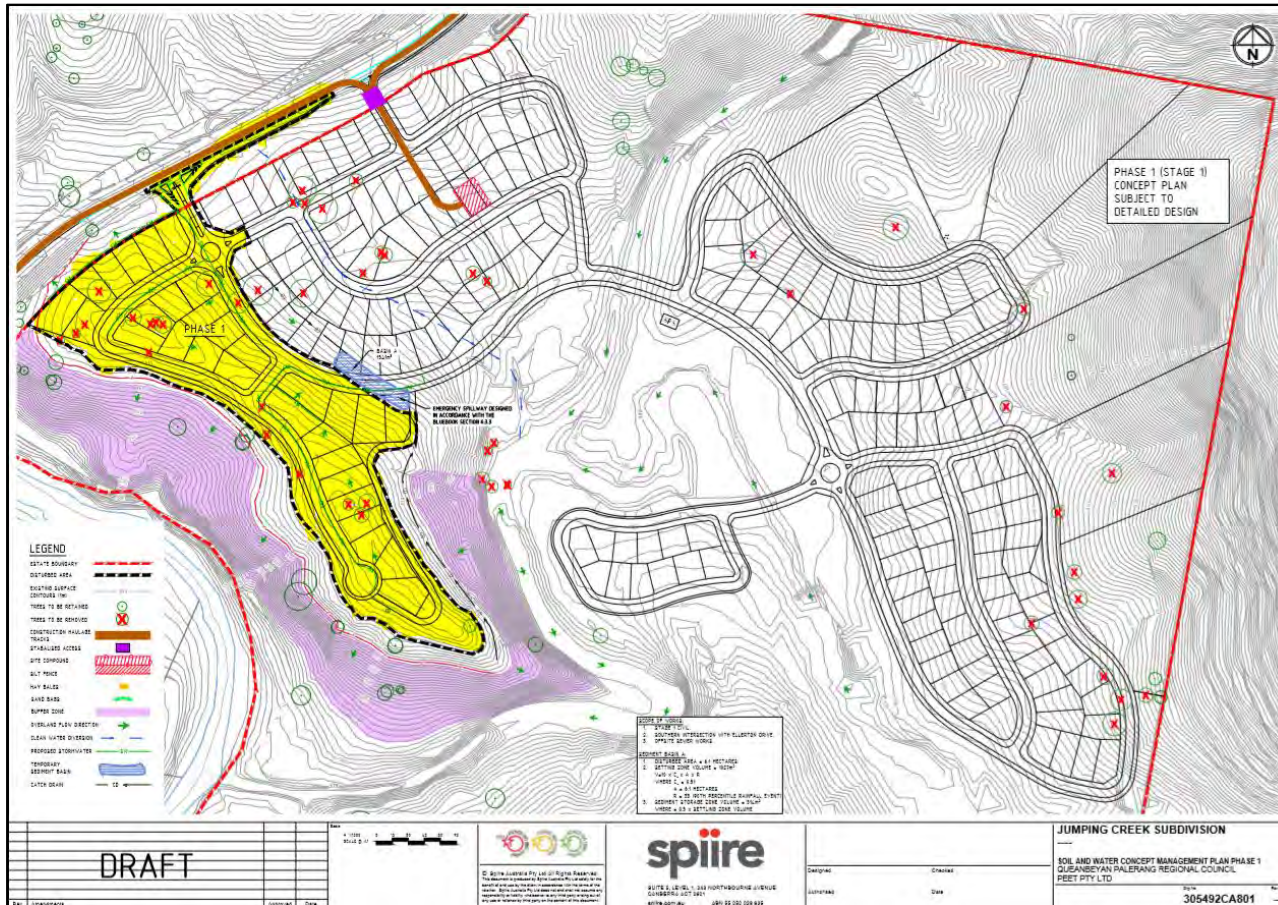
Figure 12: Soil & Water Management - Phase 1 Indicative layout only - please refer to engineering set for latest layout
