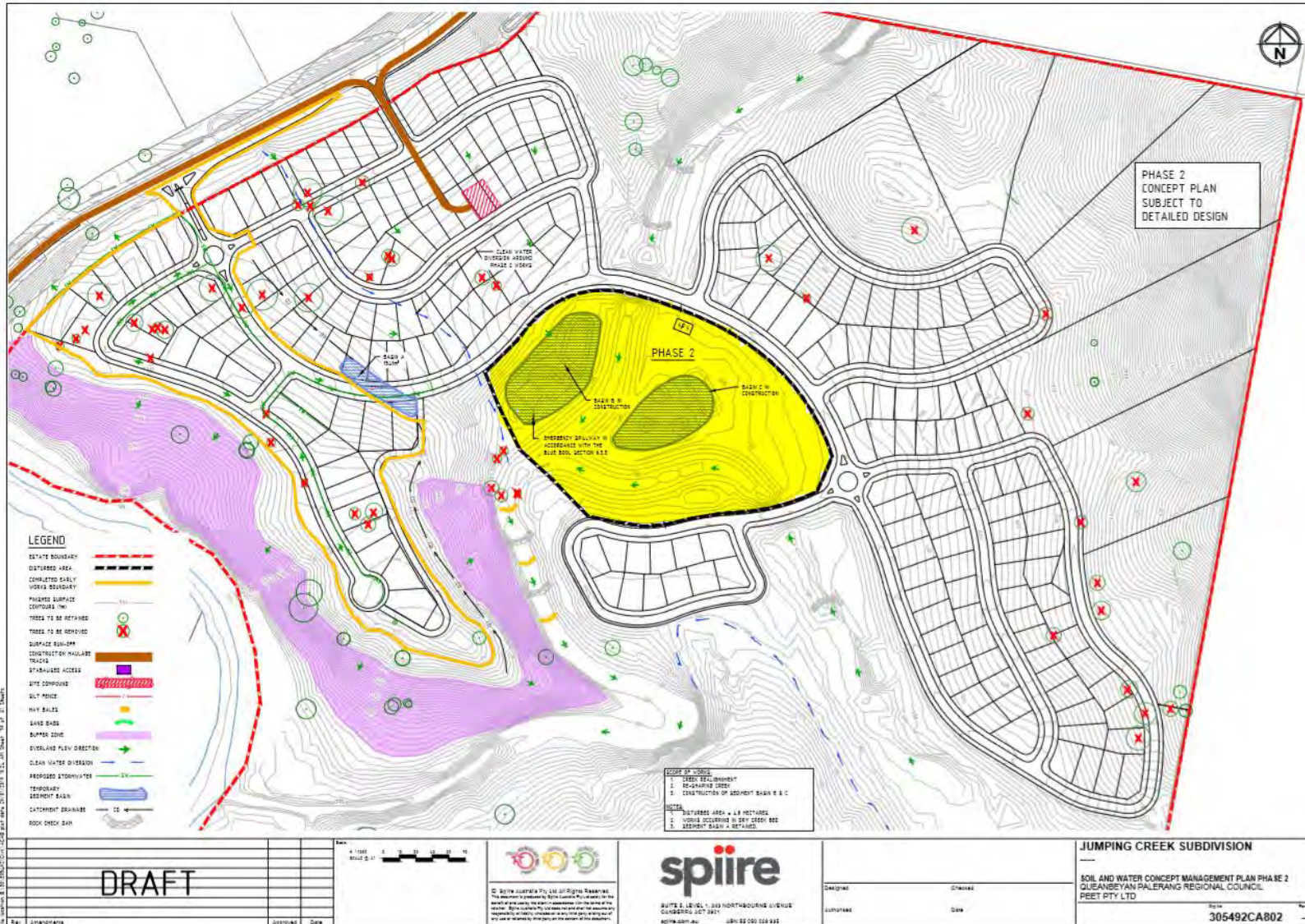
Figure 13: Soil & Water Management - Phase 2 Indicative layout only - please refer to engineering set for latest layout
