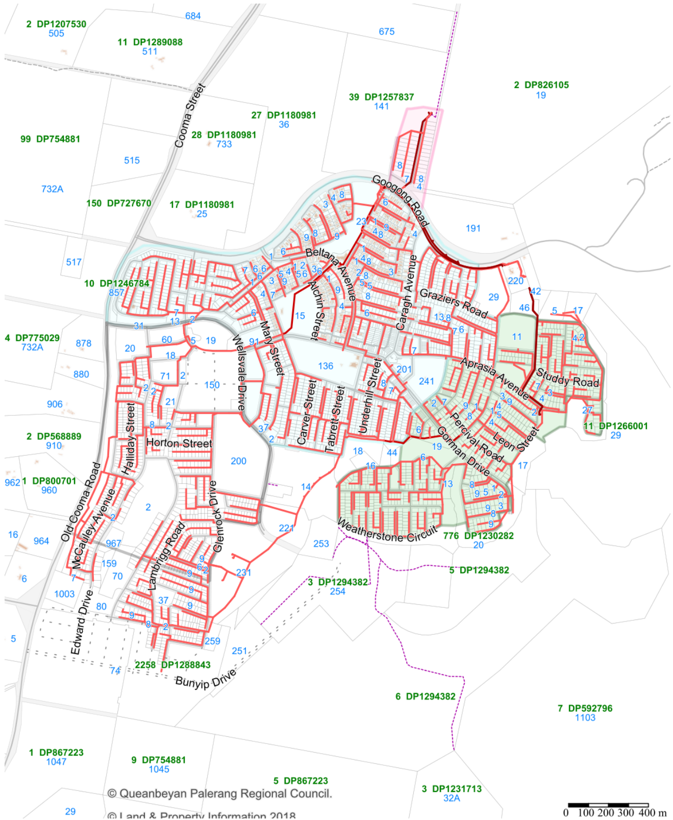
Figure 15-3 Googong Reticulation Scheme
